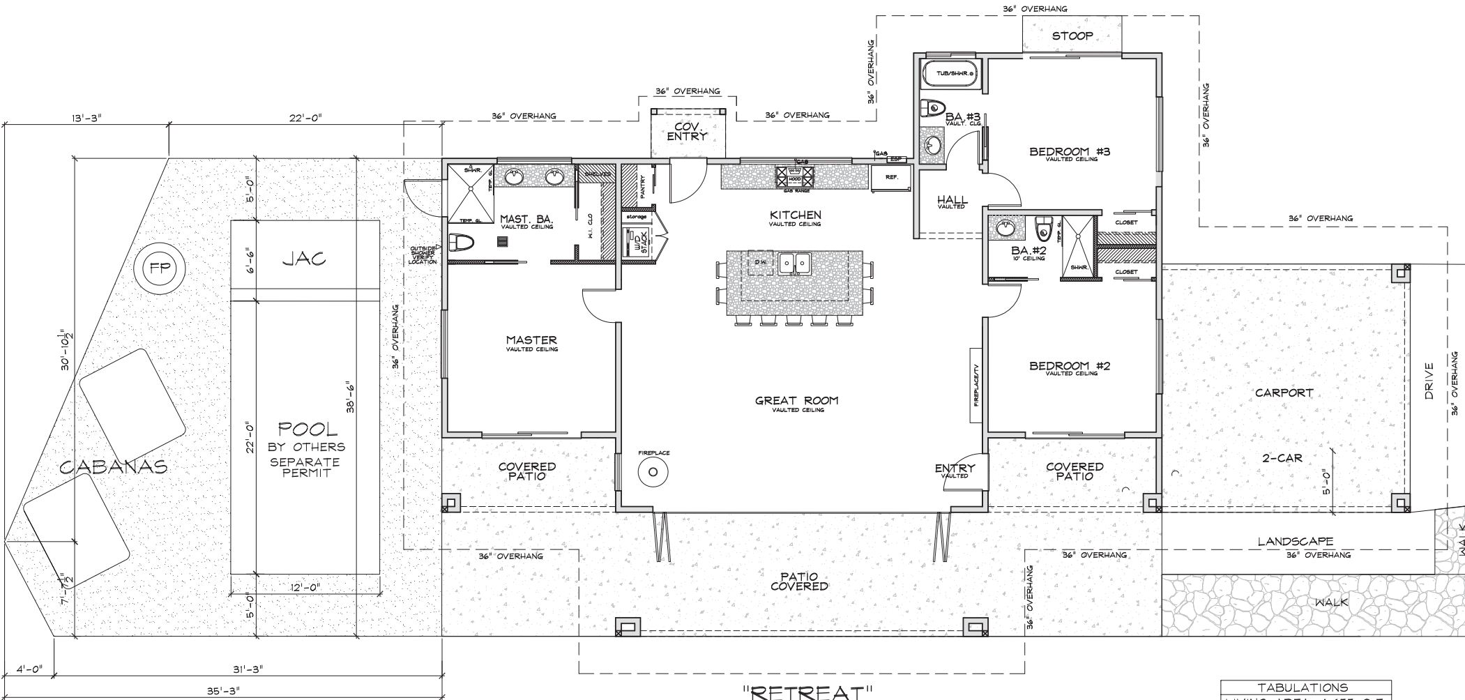
"RETREAT" FLOOR PLAN 1/4" = 1'-0" POOL AREA DIMENSIONS
